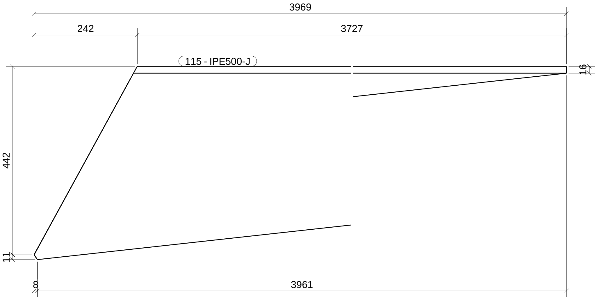
FRONT VIEW
